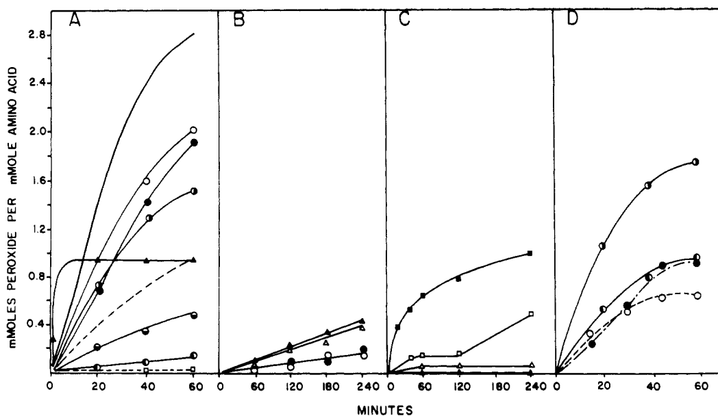
FIG. 1.—Reaction of methionine, selenocystine, and cystine derivatives with various peroxides. (A) Methionine and selenocystine with hydrogen peroxide. Cystine (0.05 M) dissolved in 2 N \text{H}_2\text{SO}_4 + 0.10 M \text{H}_2\text{O}_2 ( \square ). Selenocystine (0.05 M) dissolved in 2 N \text{H}_2\text{SO}_4 + \text{H}_2\text{O}_2 ; molarity of \text{H}_2\text{O}_2 : 0.05 ( \bullet ), 0.10 ( \ominus ), 0.20 ( \circ ), 0.30 ( \bullet ), 0.40 ( \circ ). Reaction of 0.05 M selenocystine in 88% formic acid with \text{H}_2\text{O}_2 ; molarity of \text{H}_2\text{O}_2 : 0.10 (---), 0.30 (—). Reaction of 0.05 M methionine in 2 N \text{H}_2\text{SO}_4 with 0.10 M \text{H}_2\text{O}_2 ( \blacktriangle ). (B) Methionine and selenocystine with organic peroxides. Solvent, 50% ethanol–2 N \text{H}_2\text{SO}_4 ; molarity of amino acid and of hydroperoxide, 0.05. Selenocystine + t -butyl hydroperoxide ( \circ ), selenocystine + cumene hydroperoxide ( \bullet ); methionine + t -butyl hydroperoxide ( \Delta ), methionine + cumene hydroperoxide ( \blacktriangle ). (C) Oxidized methionine or cystine derivatives with hydrogen peroxide. Amino acid (0.05 M) dissolved in 2 N \text{H}_2\text{SO}_4 + 0.10 M \text{H}_2\text{O}_2 ; either cysteic acid or methionine sulfone ( \blacktriangle ), methionine sulfoxide ( \Delta ), cystine disulfoxide ( \square ), cysteine sulfinic acid ( \blacksquare ). (D) Selenocystine with hydroperoxides in 2 N HCl. Molarity of selenocystine, 0.05. t -Butyl hydroperoxide, 0.05 M ( \circ ); cumene hydroperoxide ( \bullet ); 0.09 M \text{H}_2\text{O}_2 ( \circ ); 0.20 M \text{H}_2\text{O}_2 ( \circ ).
