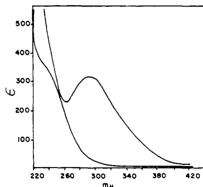
FIG. 4.—Absorption spectra of selenocystine and cystine. Amino acid (0.002 M) in 2 N H 2 SO 4 .
