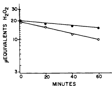
FIG. 2.—Decomposition of hydrogen peroxide by selenocystine. Selenocystine (0.05 M) + H_2O_2 (0.10 M) in 2 N H_2SO_4 (●); same reactants in 88% formic acid (○).
