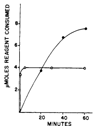
FIG. 3.—Rate of consumption of selenocystine and hydrogen peroxide. Reaction system: 0.05 M selenocystine in 2 N H_2SO_4 and 0.20 M H_2O_2 : selenocystine (○), H_2O_2 (●).
